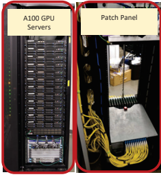
Figure 18: Testbed photo.
